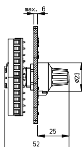
Technical drawing External Balance control kit MPM
