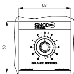
Technical drawing External Balance control kit MPM
