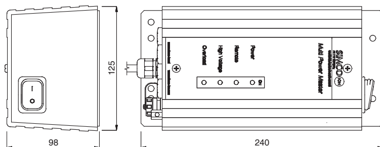
Technical drawing MPM
