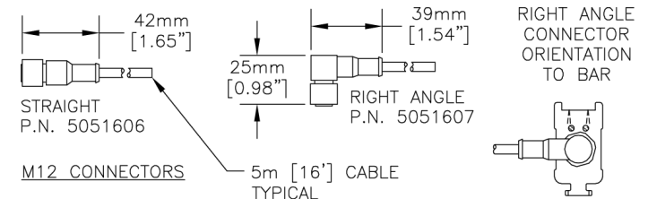
Connectors
